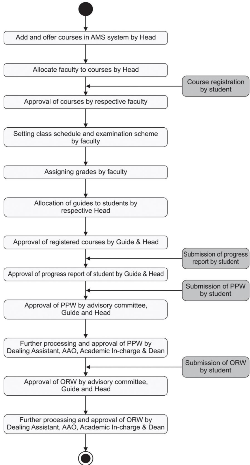
Fig. 1 Activity Diagram for Using Academic Management
